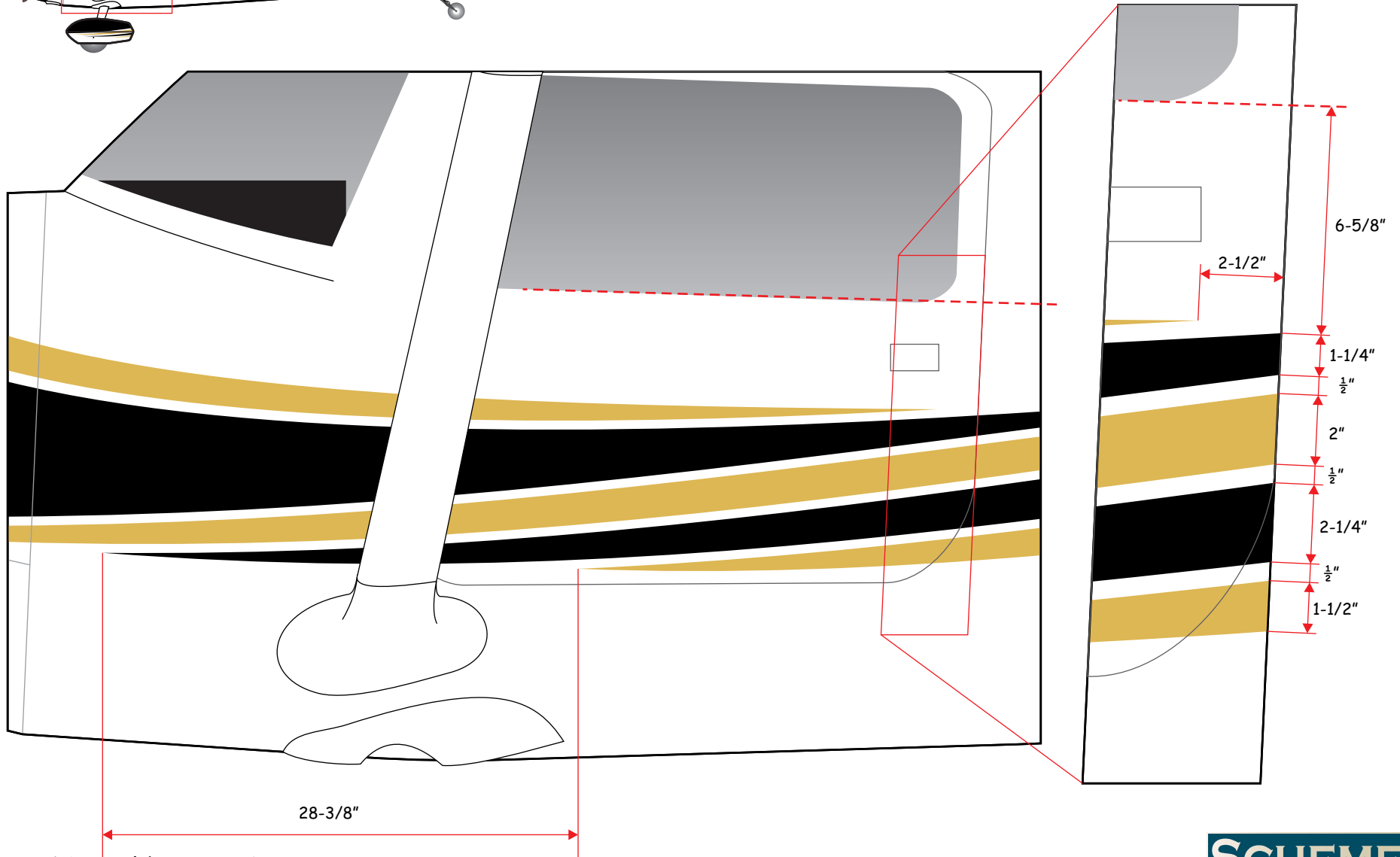
Cessna 152 Taildragger - N37ZQ Douglas Cole Cabin Door
